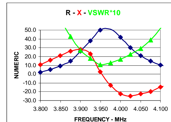
FIGURE 12 – IMPEDANCE AFTER
