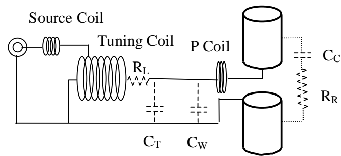
SCHMATIC DIAGRAM
